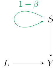
Figure 2: Recursive self-improvement explodes if and only if \beta < 0 .
