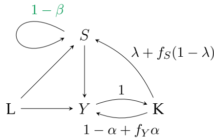
Figure 5: Economic feedback loops effectively reduce diminishing returns.
