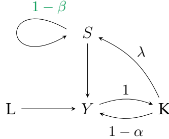
Figure 4: Economic feedback loops effectively reduce diminishing returns.
