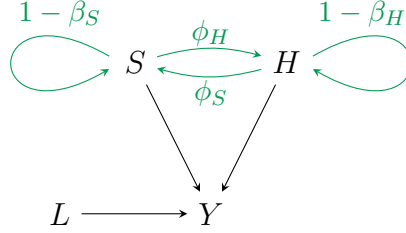
Figure 3: Innovation networks effectively reduce diminishing returns.
